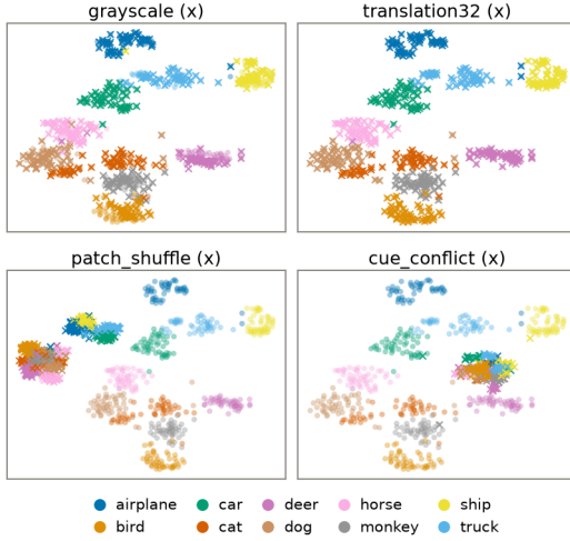
Figure 2: CLIP t-SNE: Representations overlap except in Cue Conflict and Patch Shuffle
