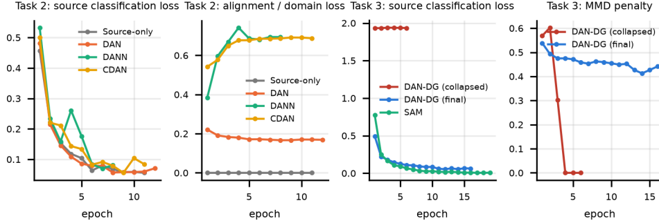
Figure 4: Training curves
